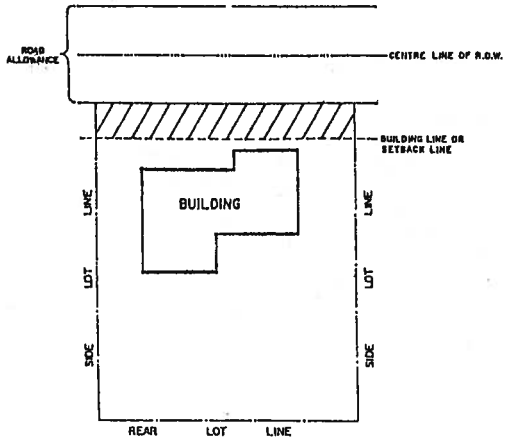
SETBACK REQUIREMENT
